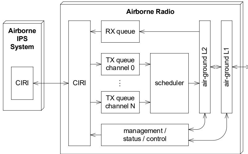
Figure 2-7 – Notional Airborne Radio Architecture
