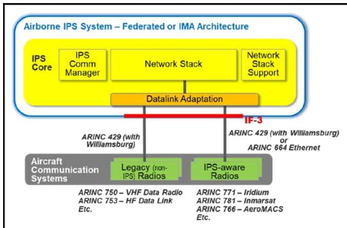
Figure 5-8 – Radio Interface in Federated or IMA Architecture
