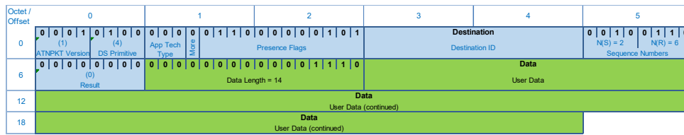
Figure A-12 – Example ATNPKT with D-ENDCNF Primitive
