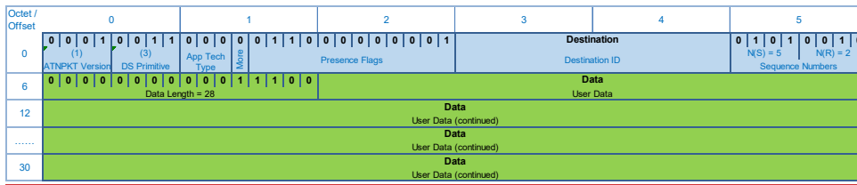
Figure A-11 – Example ATNPKT with D-END Primitive
