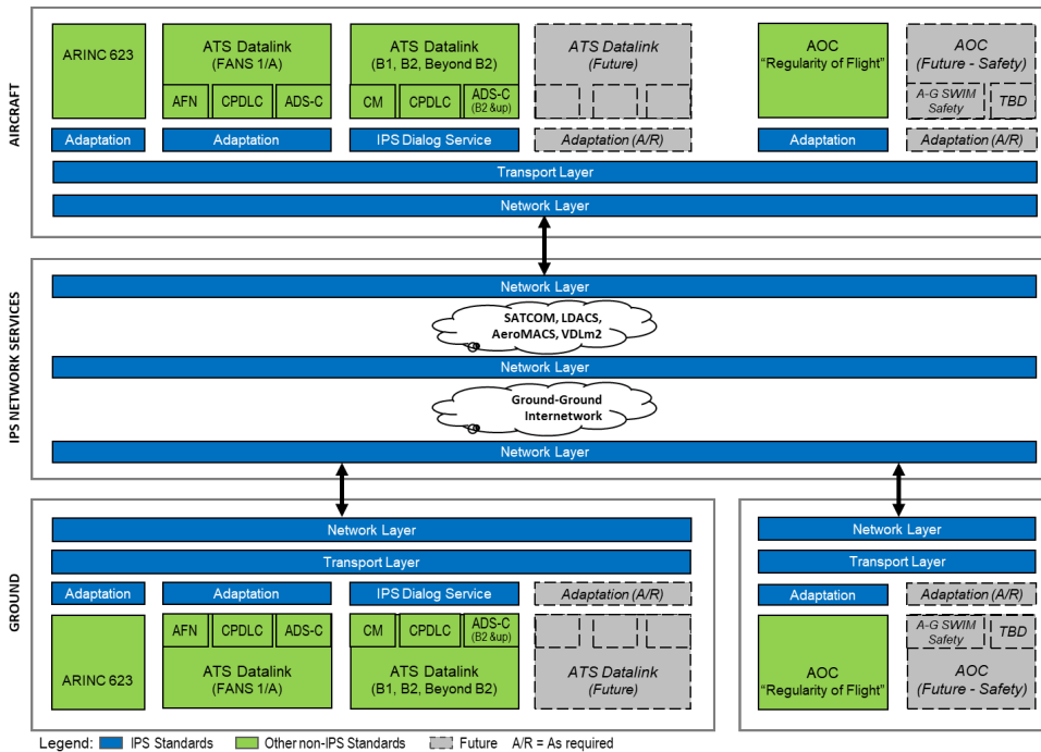
Figure C-1 – ATN/IPS Overview
