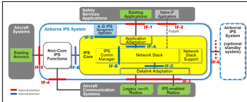
Figure 3-14 – Airborne IPS System and IPS Core External and Internal Interfaces
