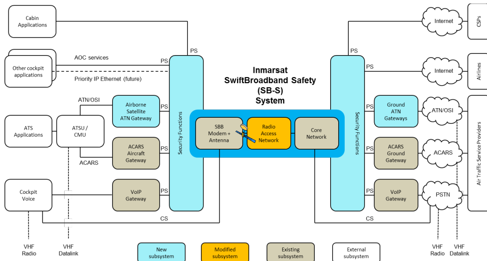
Figure C-2 – SwiftBroadband Safety High-level Architecture
