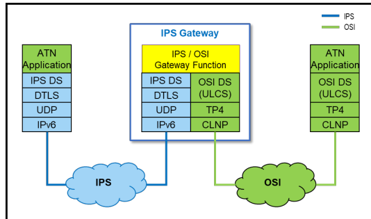
Figure 5-1 – IPS Host and ATN/OSI End System Communicating via an IPS Gateway
