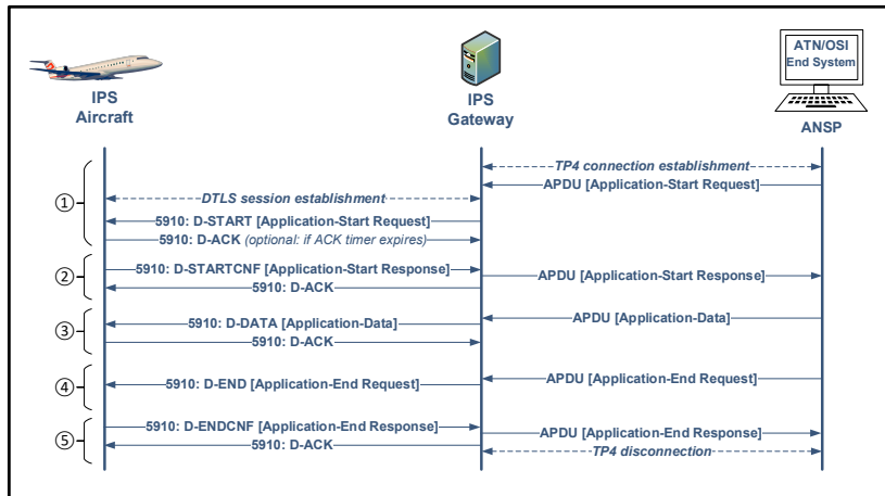
Figure 5-14 – Ground-initiated Application Message Exchanges between an IPS Aircraft and an ATN/OSI End System via an IPS Gateway
