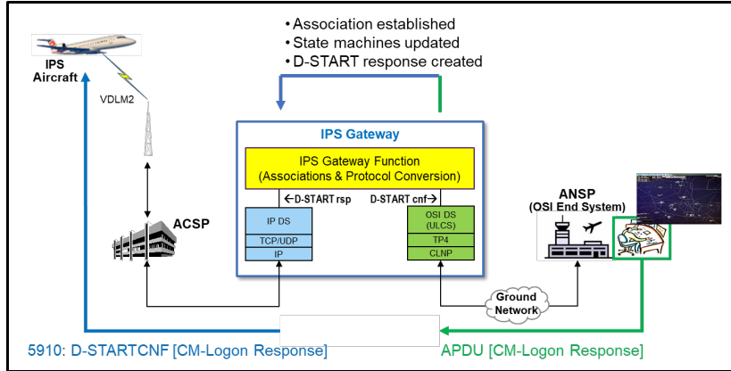
Figure 5-5 – CM Logon Uplink Response from an ATN/OSI End System to an IPS Aircraft
