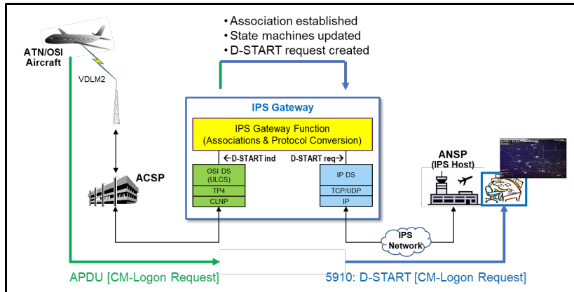
Figure 5-6 – CM Logon Downlink from an ATN/OSI Aircraft to a Ground IPS Host
