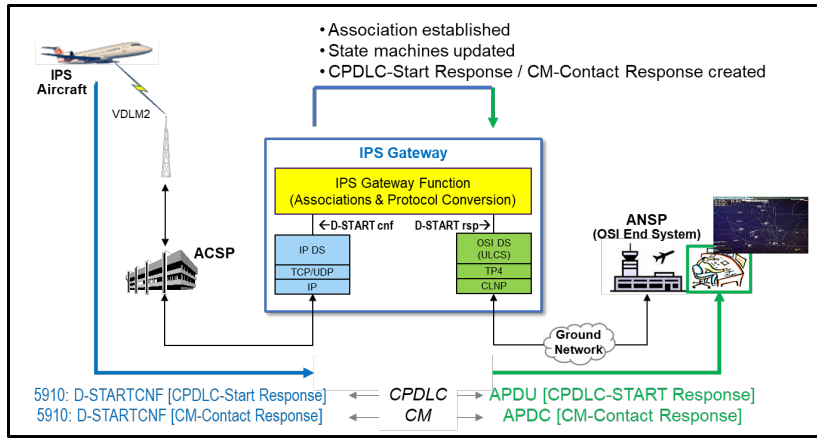
Figure 5-9 – CPDLC Start or CM Contact Downlink Response from a Ground ATN/OSI End System to an IPS Aircraft
