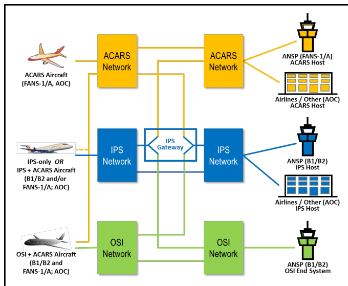
Figure 2-2 – Ground IPS System Architecture Drivers
