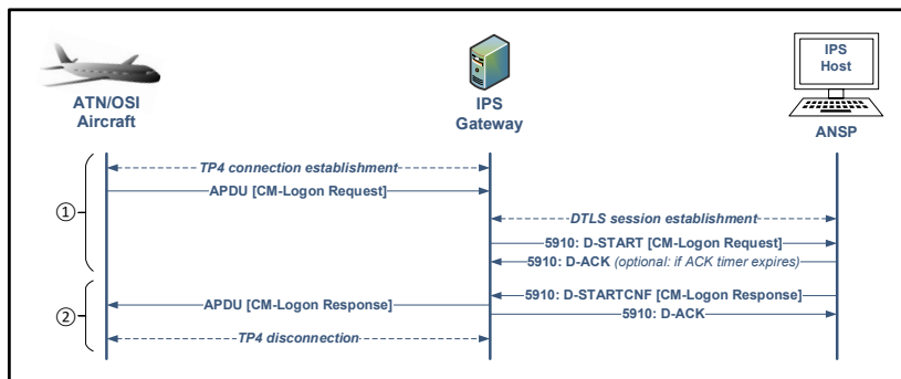
Figure 5-13 – CM Logon Message Exchanges between an ATN/OSI Aircraft and an IPS Host via an IPS Gateway
