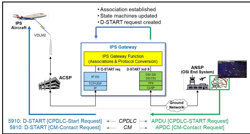
Figure 5-8 – CPDLC Start or CM Contact Uplink Request from a Ground ATN/OSI End System to an IPS Aircraft
