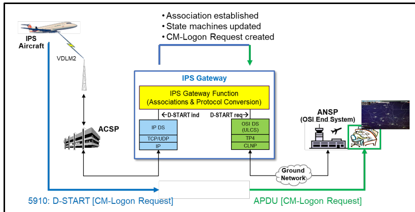
Figure 5-4 – CM Logon Downlink from an IPS Aircraft to an ATN/OSI End System
