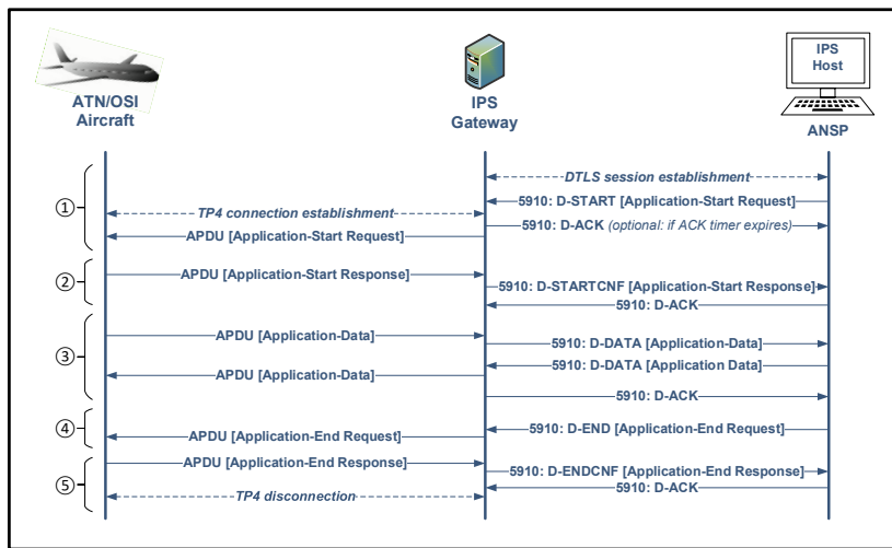
Figure 5-15 – Ground-initiated Application Message Exchanges between an ATN/OSI Aircraft and a Ground IPS Host via an IPS Gateway
