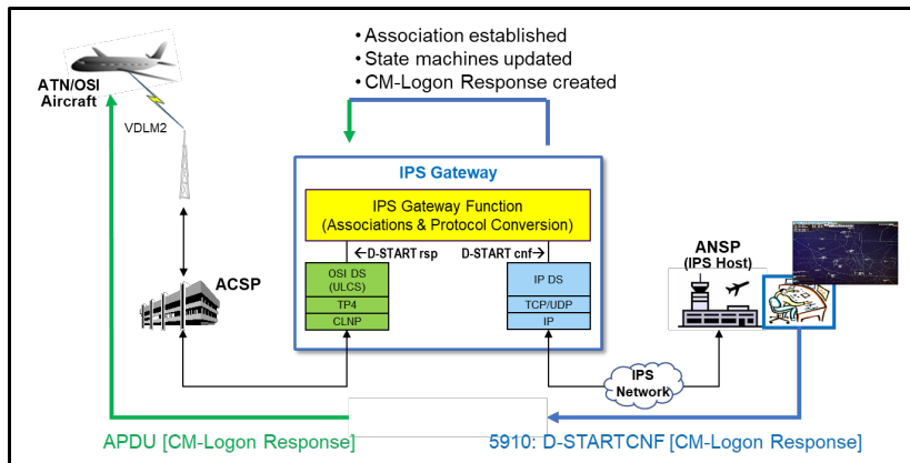
Figure 5-7 – CM Logon Uplink Response from a Ground IPS Host to an ATN/OSI Aircraft
