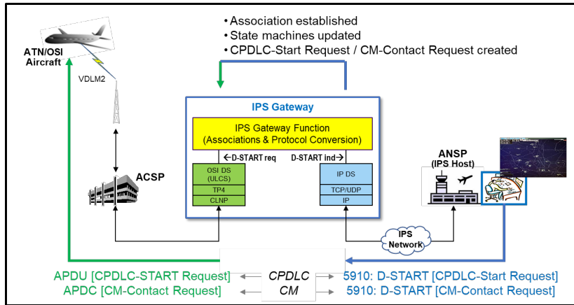
Figure 5-10 – CPDLC Start or CM Contact Uplink Request from a Ground IPS Host to an ATN/OSI Aircraft
