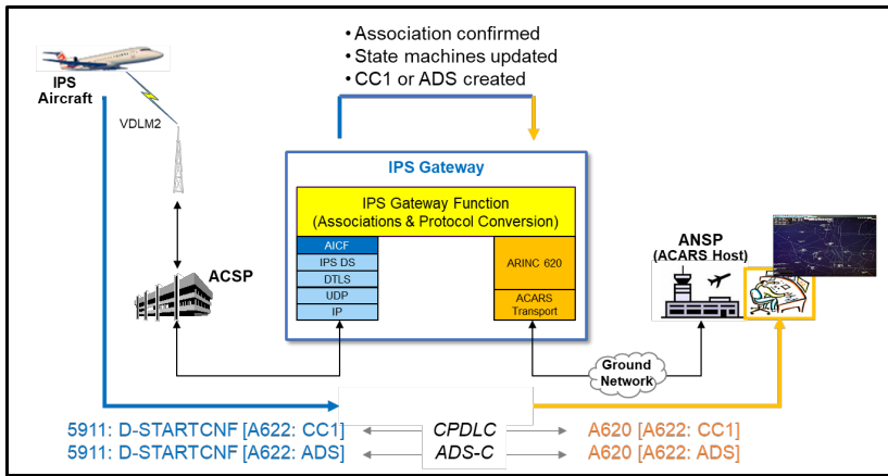
Figure 4-10 – FANS-1/A CPDLC or ADS-C Downlink (No Existing Dialogue)
