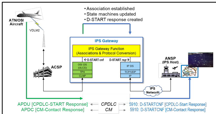
Figure 5-11 – CPDLC Start or CM Contact Downlink Response from a Ground IPS Host to an ATN/OSI Aircraft
