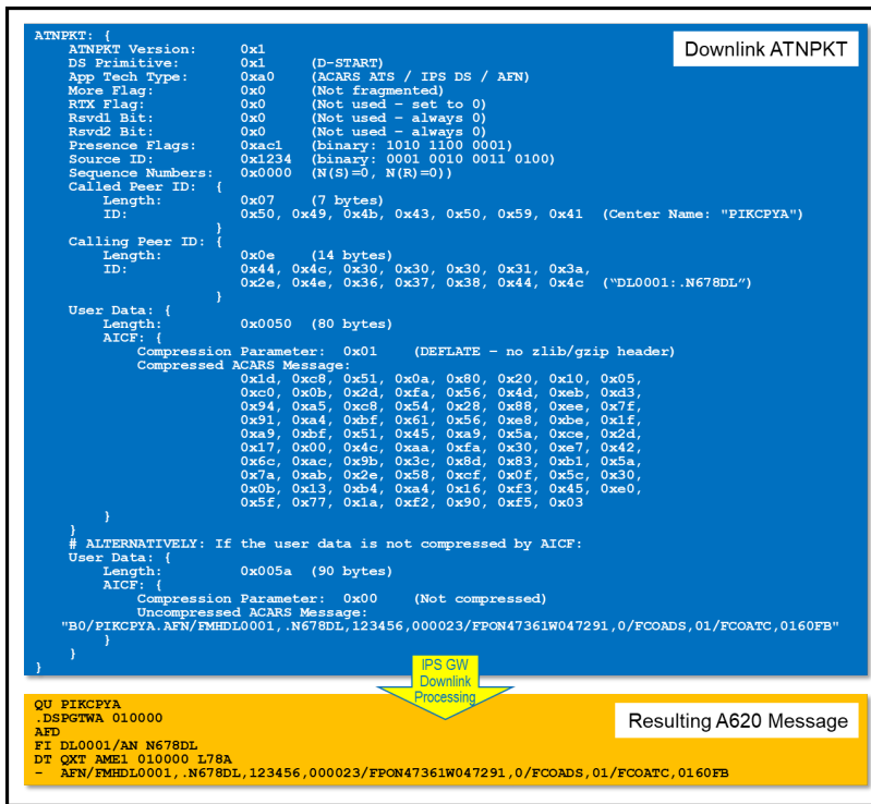
Figure 4-2 – ARINC 620 Downlink Message Conversion Example
