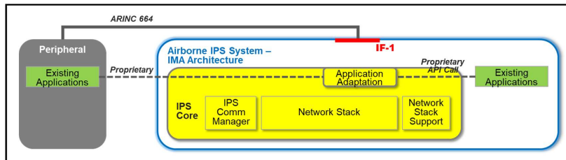
Figure 5-7 – Existing Application Interface in an IMA Architecture
