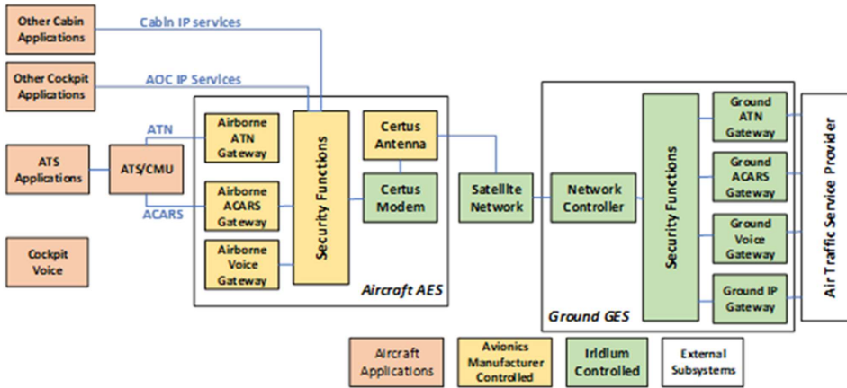
Figure C-3 – Iridium Certus Safety High-level Architecture
