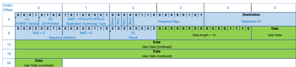
Figure A-12 – Example ATNPKT with D-ENDCNF Primitive
