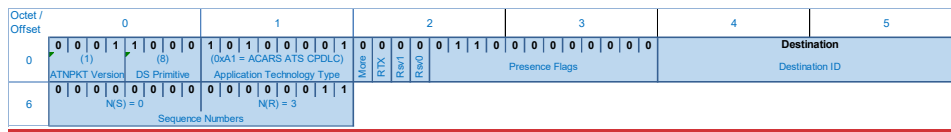
Figure A-10 – Example ATNPKT with D-ACK Primitive
