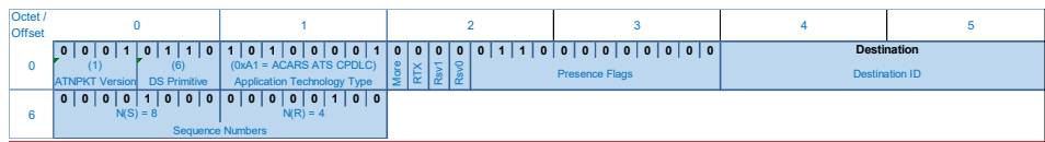
Figure A-13 – Example ATNPKT with D-ABORT Primitive
