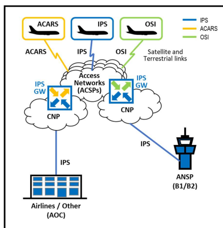
Figure 2-6 – IPS-only Ground Host Deployment
