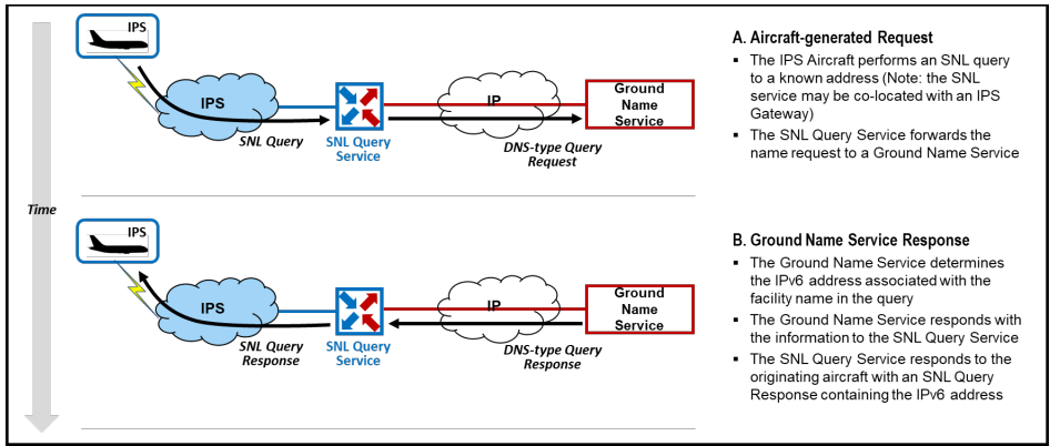
Figure 3-13 – Aircraft Acquisition of Ground Address
