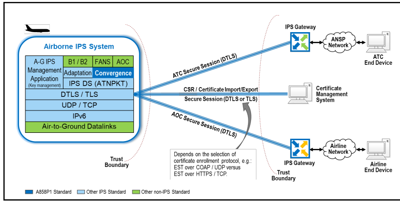
Figure 4-4 – Rekeying using a DTLS-Dedicated Secure Session with a Certificate Management System
