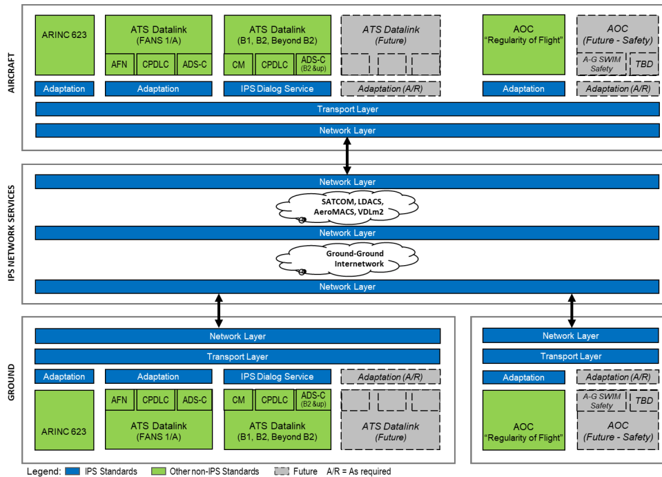
Figure C-1 – ATN/IPS Overview
