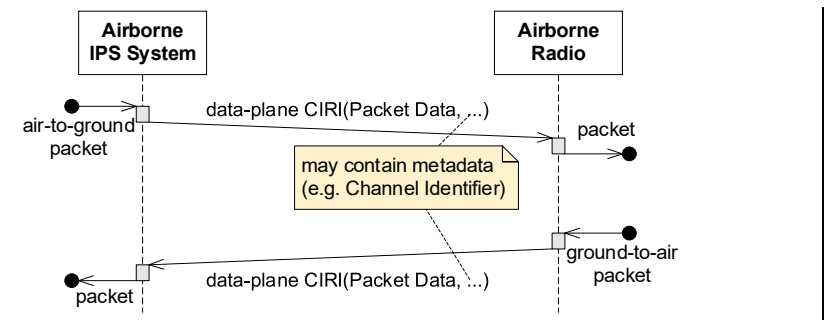
Figure 2-5 – Data Plane Communication Pattern
