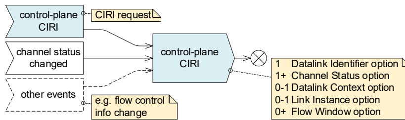
Figure 4-3 – Airborne Radio CIRI Endpoint Control Plane Operation
