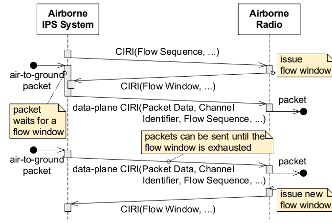
Figure 2-6 – Flow Control Example Sequence
