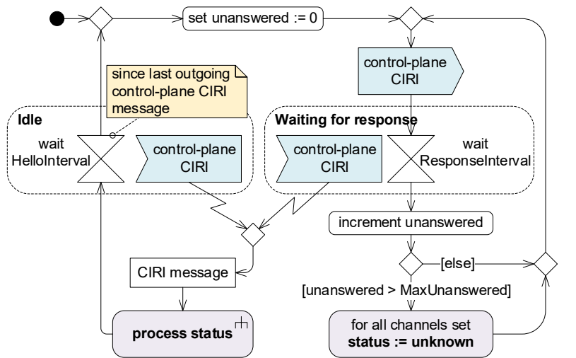
Figure 4-1 – Airborne IPS System Endpoint Control Plane Operation
