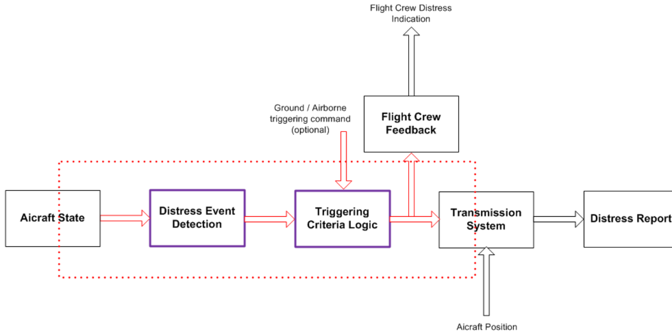
Figure 35: ADT functional architecture.
